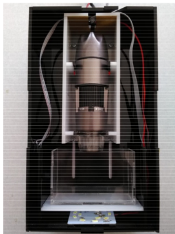
Fig 3. Realization of measurement chamber
