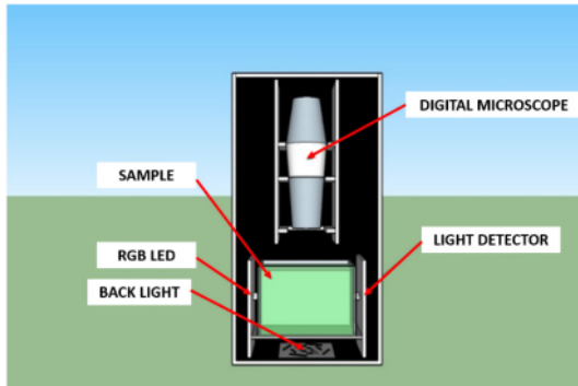
Fig 2. Measurement Chamber
